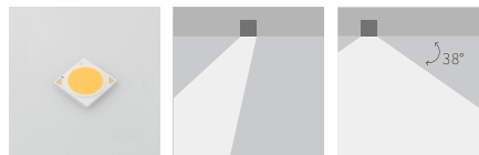
COB LED(CREE) ADJUSTABLE CUT-OFF ANGLE 38°
