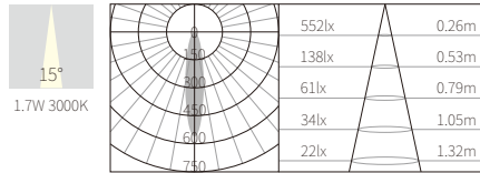
LED FIXED
