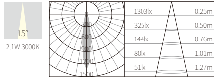
LED(CREE)
