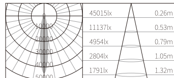
COB LED(CITIZEN)
